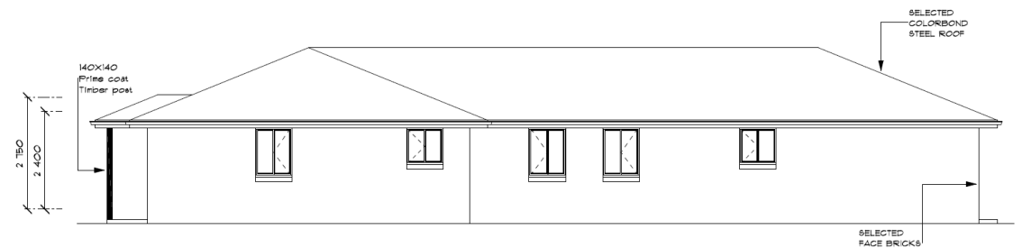
SOUTHWEST ELEVATION
