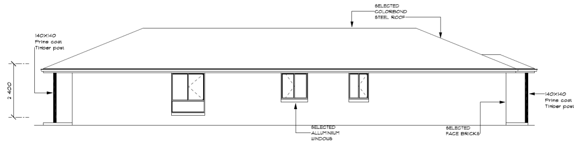
NORTHEAST ELEVATION
